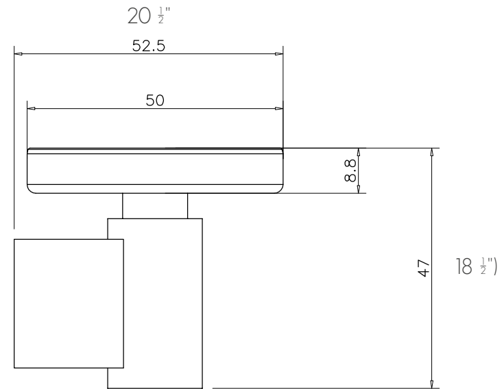
LATERAL / SIDE
