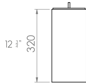
FRONTAL / FRONT
