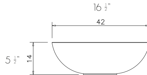
LATERAL / SIDE
