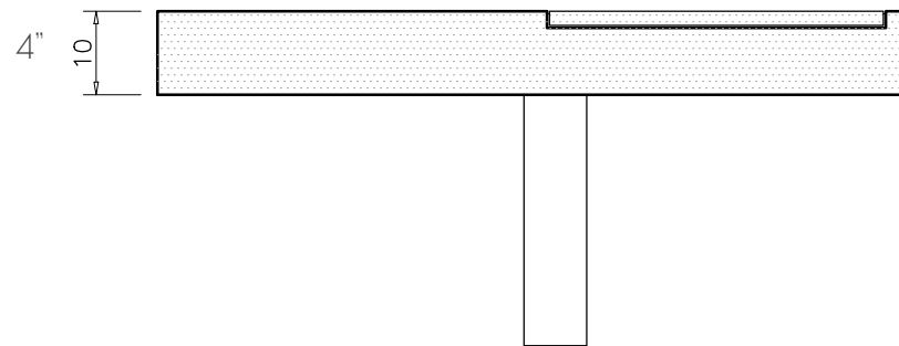
FRONTAL / FRONT
